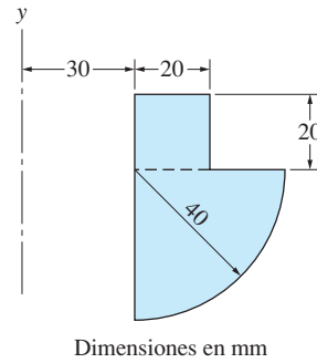
Fig. P8.127, P8.128
