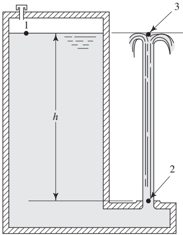
FIGURA 6.11 Chorro vertical.
