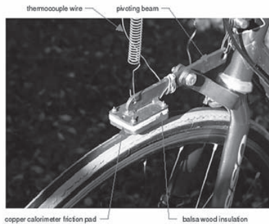
Figure 9.1 The copper calorimeter friction pad used for braking a bicycle.
