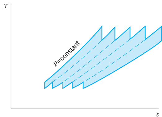
FIGURE 12.7 T-s diagram that shows how the gas-turbine cycle with many stages approaches the Ericsson cycle.
