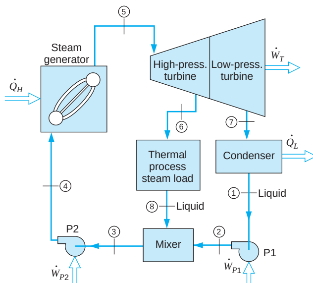
FIGURE 11.19 Example of a cogeneration system.
