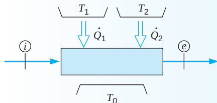
FIGURE 10.6 The feedwater heater for Example 10.1.
