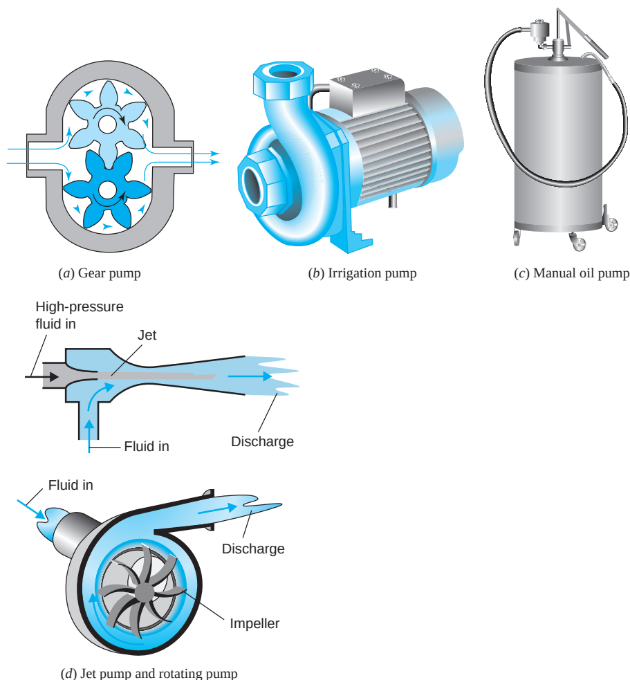
FIGURE 6.20 Liquid pumps.
