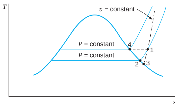
FIGURE 13.3 T – s diagram to show definition of the dew point.
