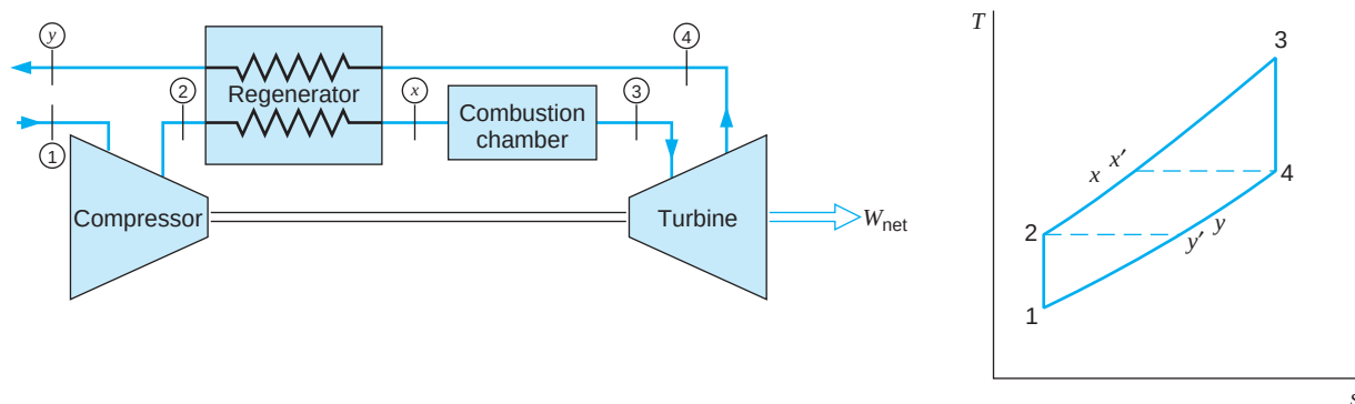
FIGURE 12.5 T - s diagram illustrating the definition of regenerator efficiency.
